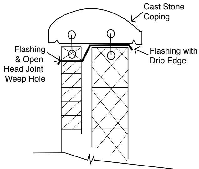
DETAIL 3: Flashing at Copings/Caps
