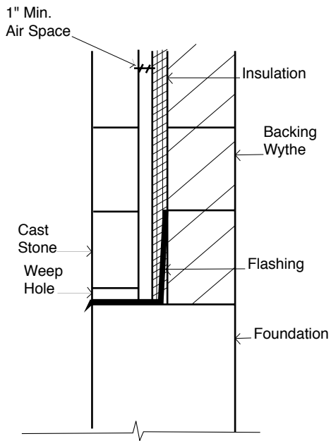
DETAIL 1: Flashing at Base
