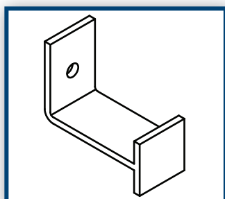
STA-09: "L" ANCHOR WITH WELDED TAB
